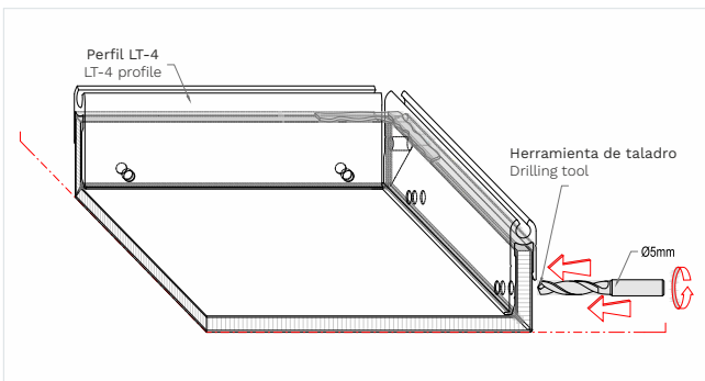
Drilling of the panel through its external face to fix in the panel of the waterproofing rivets.
