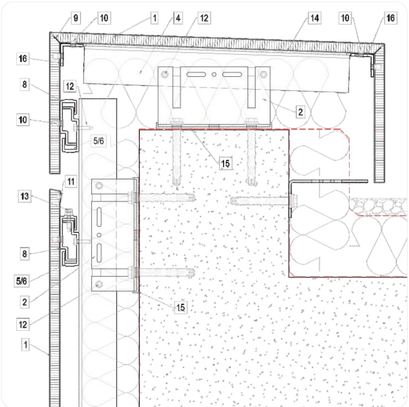
7. Parapet detail
