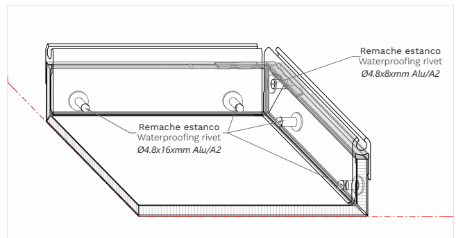
Cassette finished and ready to install with Hidetech® LIGHT installation system.
