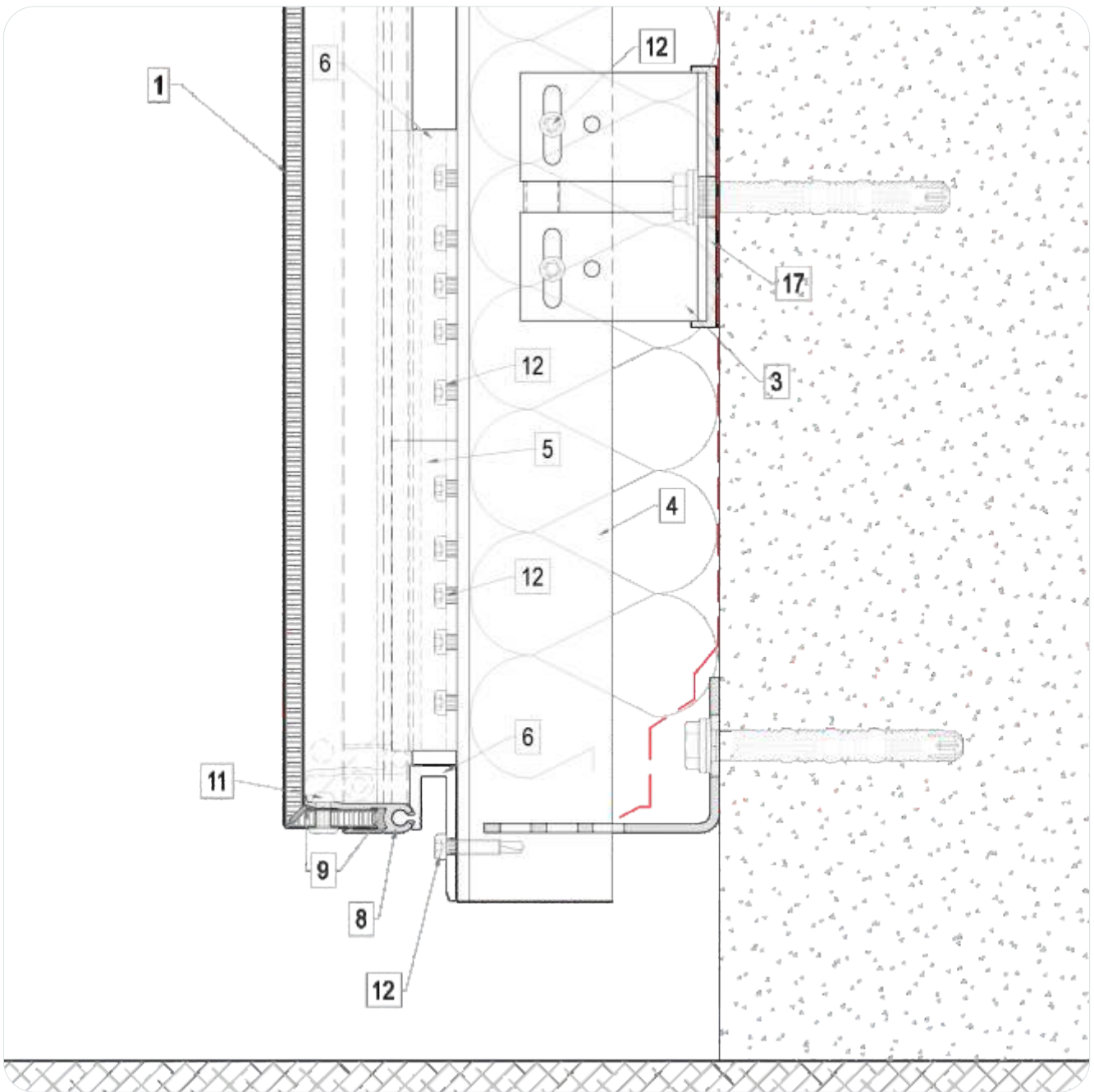
05b. Facade starting II
