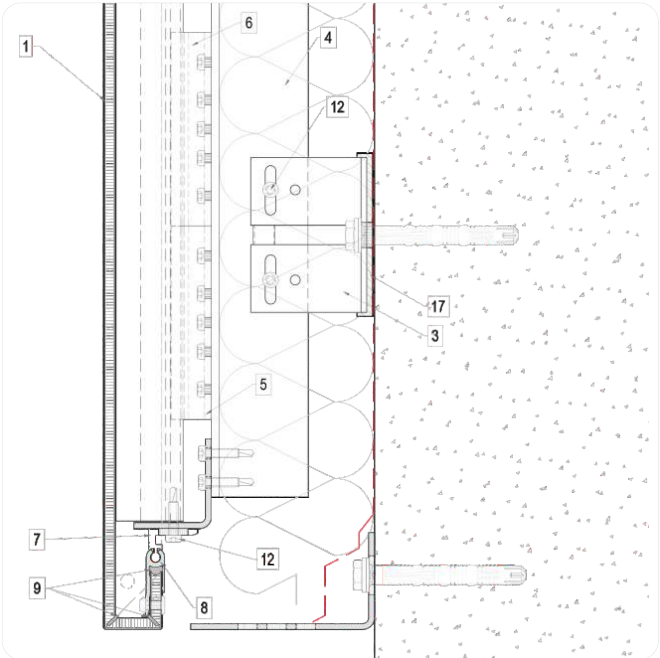
06a. High façade starting I
