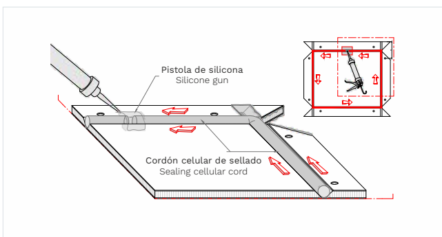
Sealing silicone and placed of the cellular cord. Sealing the joint of the ends of the cellular cord
