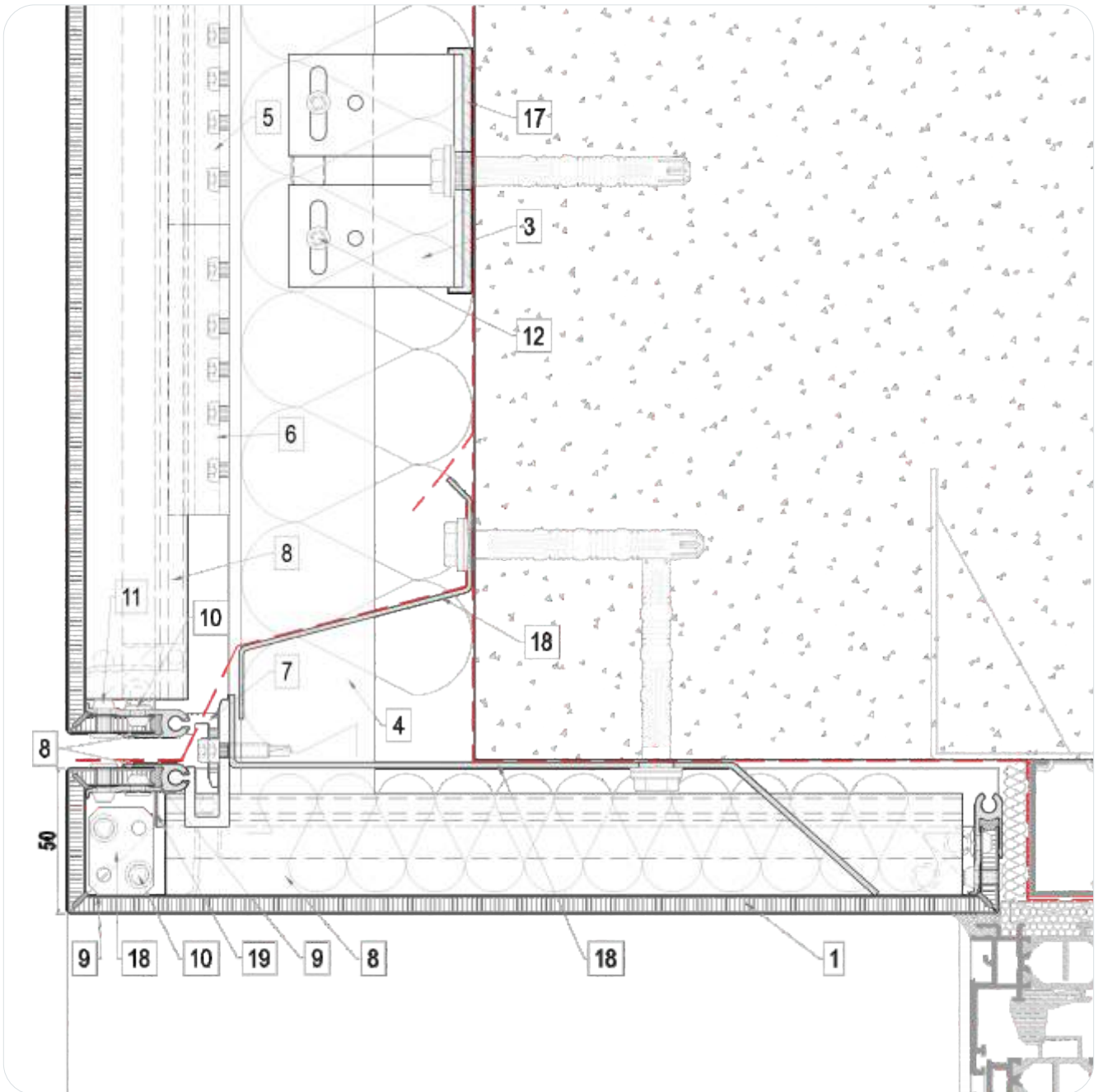
09. Window head detail
