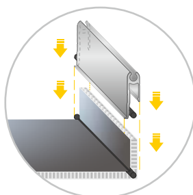
5. Insert LT-4 profile with cellular cord
