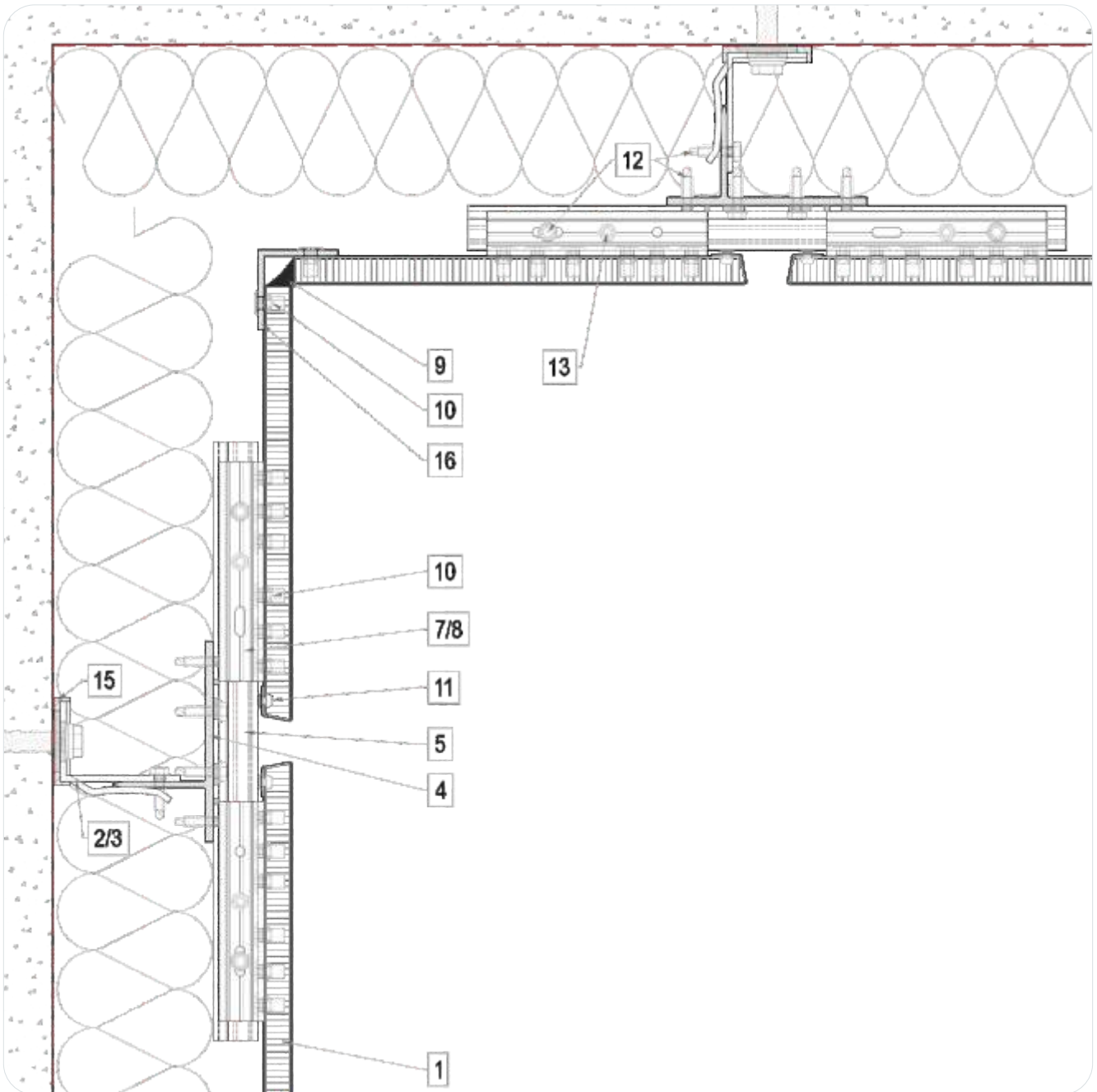
8b. Internal corner
