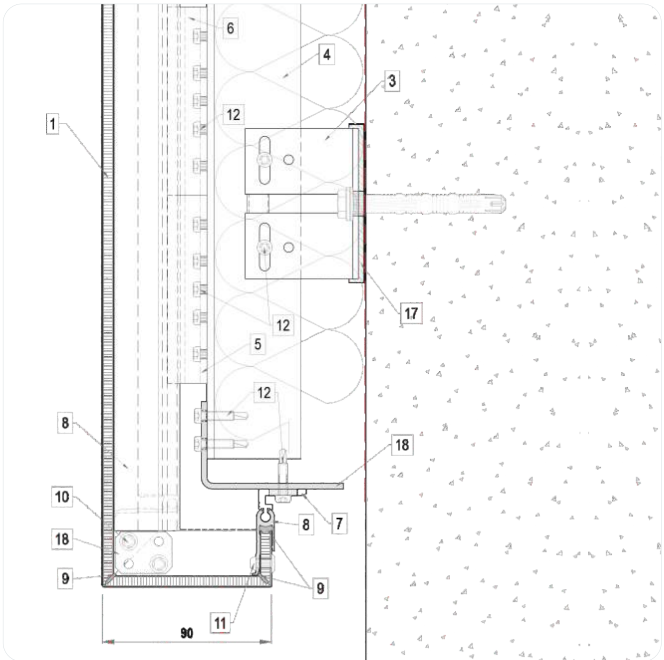
06b. High façade starting II
