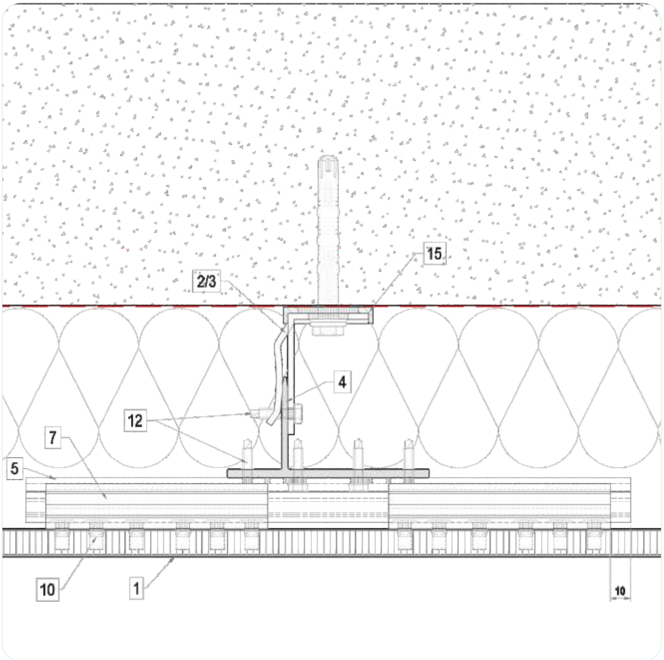
3b. Intermediate long hanger with bracket LT-1A/B 60-160
