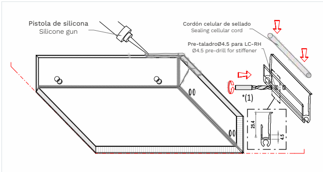
Sealing silicone is applied to cassette corners. Placement of the cellular cord inside of LT-4 profile.
