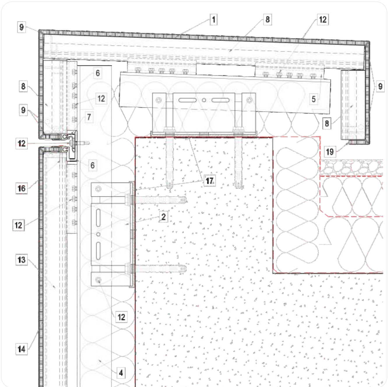
07. Parapet detail
