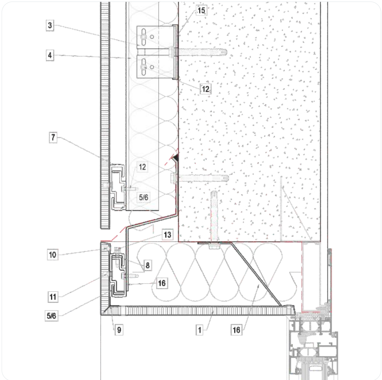
9. Window head detail
